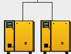
Connection of compressors with SIGMA CONTROL; connection to stations with SIGMA network (SAM 1 alternative)
